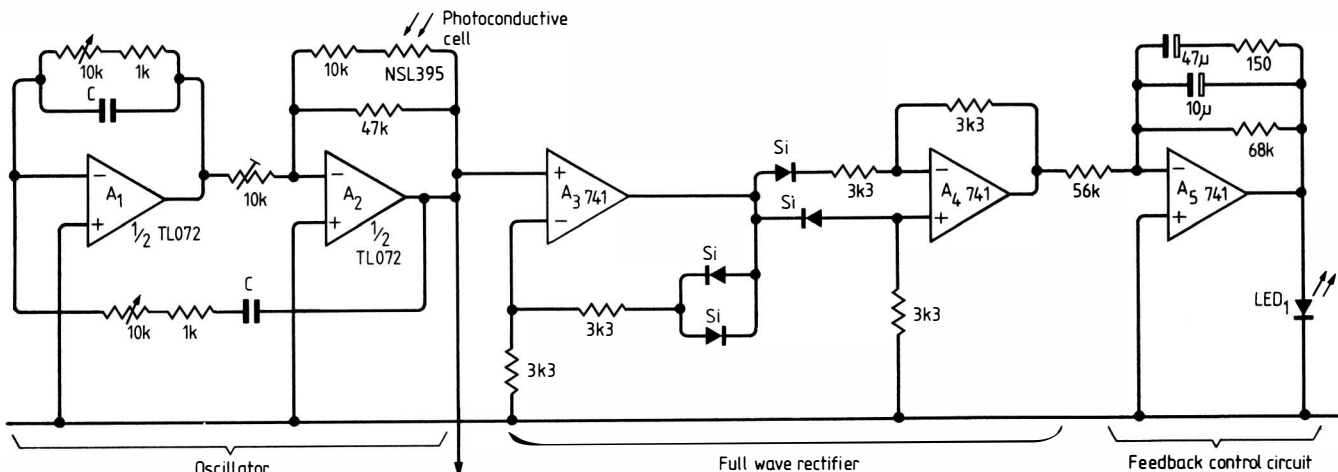
Note: PC 1 and LED 1 are in optical contact
