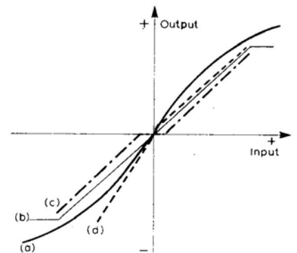
Fig. 6 (right) Typical transfer characteristics of audio circuits: (a) S-type characteristic (b) op-amp type of characteristic (c) circuit with cross-over distortion; and (d) t.h.d. constant with applied signal level.
