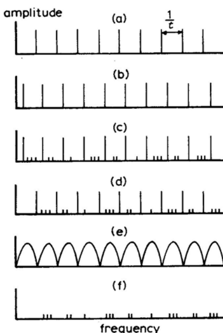
Fig. 1. Spectra illustrating principle of the single comb-filter distortion measurement method: (a) spectrum of pseudo-random binary sequence; (b) the same p.r.b.s. frequency shifted; (c) signal from system under test, showing distortion products in gaps; (d) signal re-shifted; (e) response of comb-filter for removing comb spectrum of p.r.b.s. test signal; and (f) comb-filter output. T is repetition period of p.r.b.s.)
