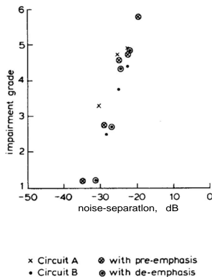
Fig. 7 (below). Plotted points showing good correlation between subjective average impairment grade and measured noise-separation in the double comb-filter method, with two circuits A and B. Note that points are closely grouped when compared with those in Fig. 8.
