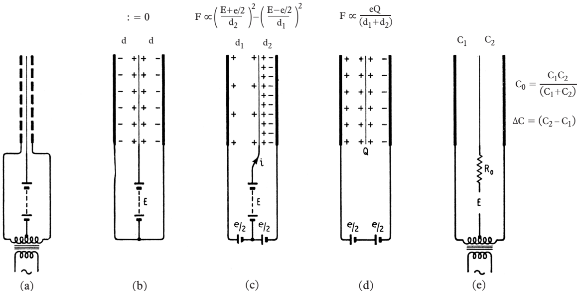
Fig. 1. Essential differences in the operation of electrostatic loudspeakers with "constant voltage" and "constant charge" on the centre diaphragm.
