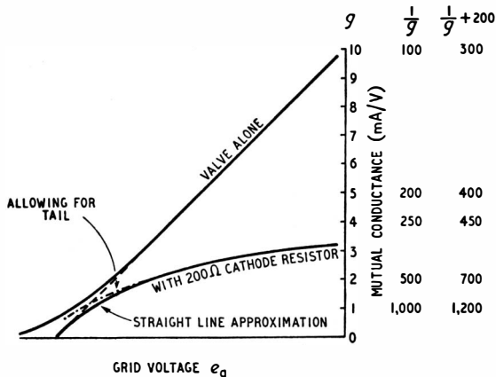
Fig. 3. The use of an unbypassed cathode resistor makes the effective mutual conductance more constant, but adds higher-order terms to the valve characteristic.
