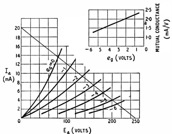
Fig. 6. For a triode it is necessary to fix the load line before plotting the g_m - e_g characteristic. This typical example shows a linear g_m - e_g characteristic for R_L = 12,500 ohms.
