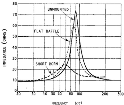
Fig. 2. Effect of loudspeake mounting on impedance of voice coil.
