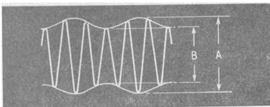
Fig. 4. Form of trace obtained with circuit of Fig. 3.
