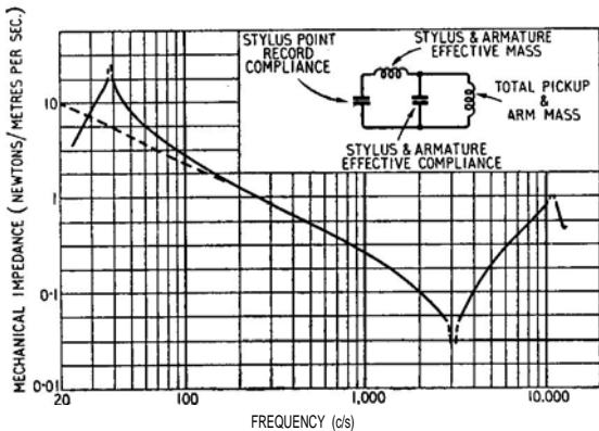
Fig. 1. Variation with frequency of the mechanical impedance at the needle top of a popular commercial pickup (1 Newton = 105 dynes).
