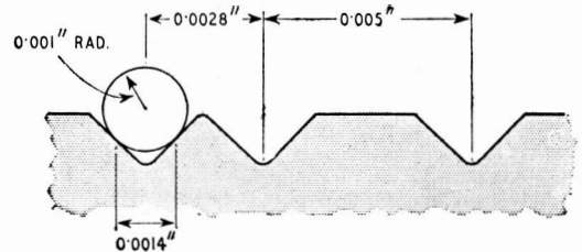
Above: Fig. 3. Using the groove of Fig. 2, the theoretical minimum spacing without modulation is 0.0028in (about 350 grooves per inch). In practice an average of 250 g.p.i. is rarely exceeded.
