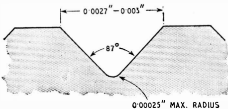
Fig. 2. Principal groove dimensions in micro-groove recording.
