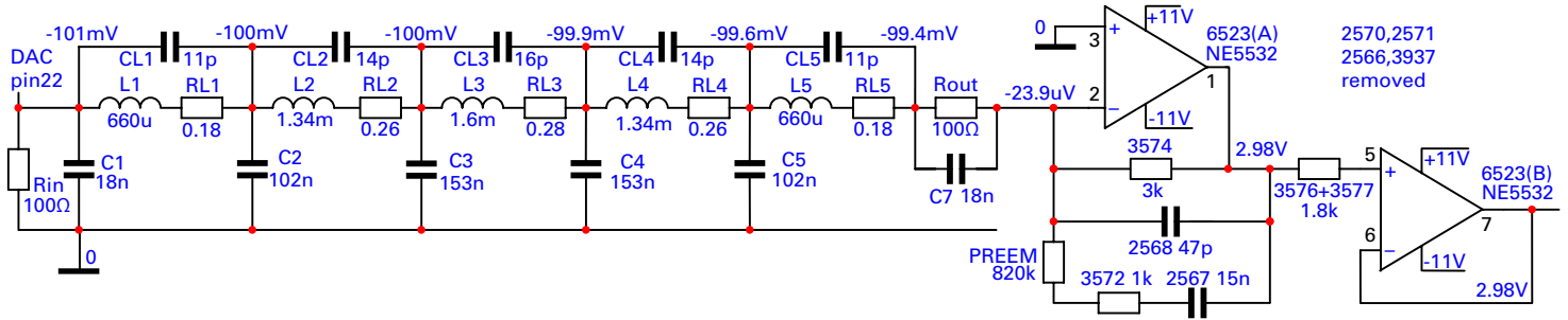
Marki microwave 11th Order Butterworth Lowpass Cutoff Frequency = 20.00 kHz
