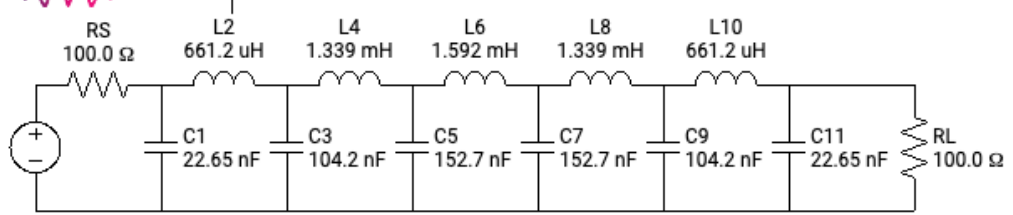
Marki microwave 11th Order Butterworth Lowpass Cutoff Frequency = 20.00 kHz
