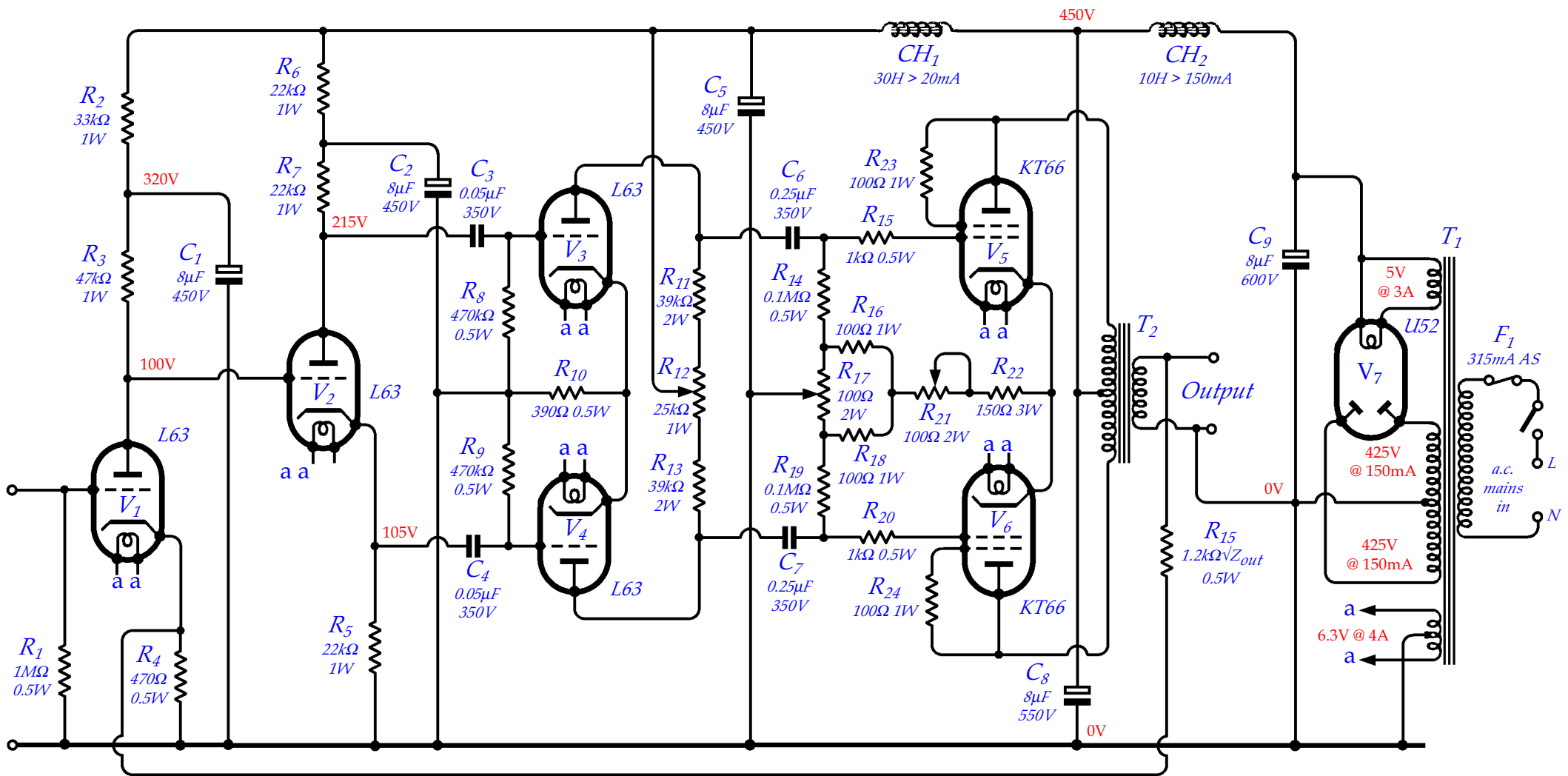
Design for a high Quality Amplifier " The Williamson Amplifier " from Wireless World May 1947 p. 161 Redrawn in original form by Keith Snook d.c. ~ daylight ltd.
