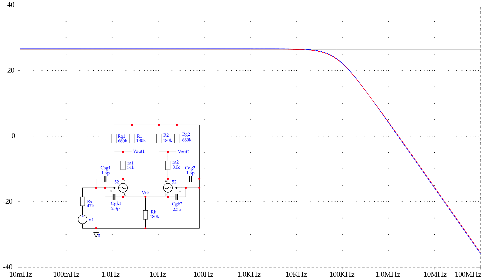
(A) triode cathode coupled phase split.dat
